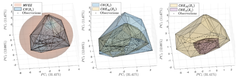
Figure 2: Comparison of the hypervolumes generated by the MVEE, CH, and CHE approaches for the species Bbar with n = 3 .
