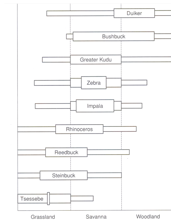
Fig. 9.10 Habitat partitioning and overlap by ungulates in Kyle National Park, Zimbabwe. The width of the boxes reflects the degree of preference. (After Ferrar and Walker 1974.)
